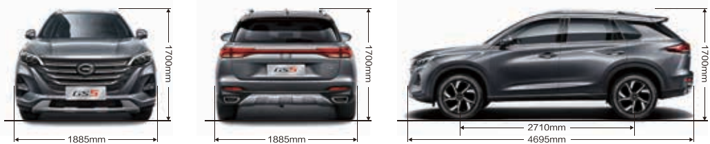
Three views
